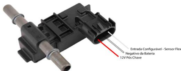
ACDelco 13577429 Sensor Flex Fuel
